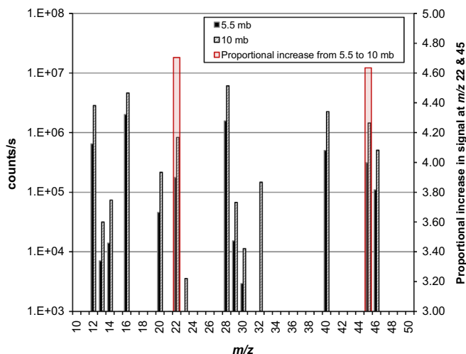
Fig. 1. Spectra from calibration experiments with the SAM breadboard QMS at 5.5 and 10 mb. Red boxes overlying the spectra illustrate the disproportionate increase with pressure of ions observed at m/z 22 compared to m/z 45. Note that there is no signal at m/z 44, the major isotopologue of \text{CO}_2 , due to detector saturation. Some m/z shown reflect contributions from other components in the Mars mix gas. (For interpretation of the references to color in this figure legend, the reader is referred to the web version of this article.)
