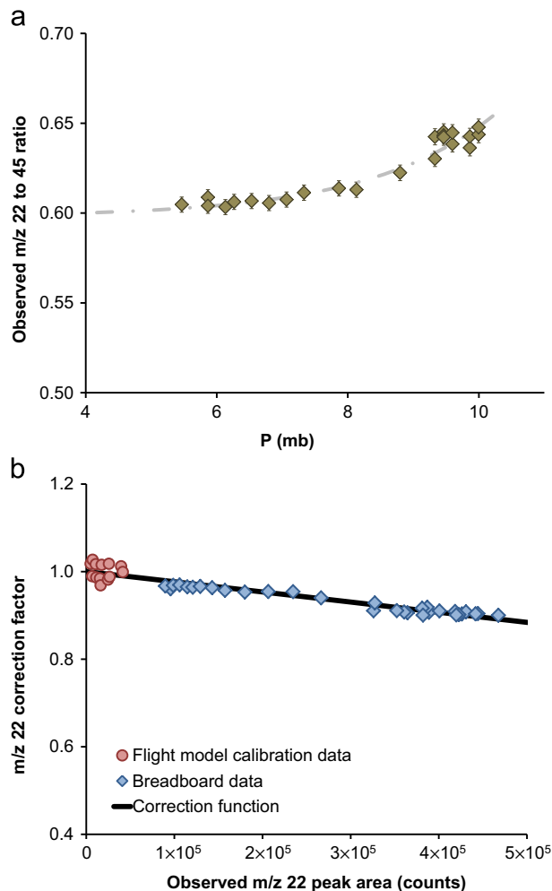
Fig. 2. (a) Illustration of growth in the ratio between m/z 22 and 45 with pressure in breadboard experiments, suggesting an increase in production of \text{CO}_2^+ ions in the QMS source. This effect is not interpreted as an isotopic fractionation because the ratio between m/z 45 and 46 remained approximately constant with pressure. (b) Correction function derived from combined flight model and breadboard data. Data shown reflect fractional scan peak areas. Error bars reflect effects of statistical noise and dead time correction for the observed signal, propagated through calculations of background subtraction and isotope ratios. Error bars in (b) are smaller than the symbols.
